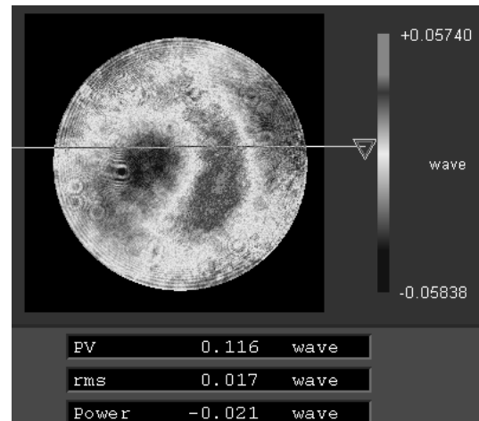
Fig. 4 The average of the four contour maps in Fig. 2, that is, the error in the f/3.3 transmission sphere
