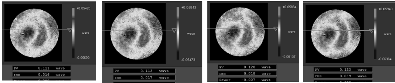
Fig. 2 Contour maps of the test of the random ball in four different test patches P-V ranges from .111 to .123 \lambda and rms from .016 to .019 \lambda
